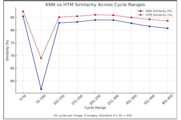
Fig. 6. Similarity Graph
